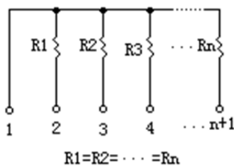
A TYPE(Bussed)
