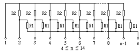
RTYPE(Dual Terminator)
